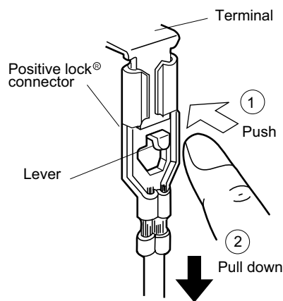
Figure C-1. Positive Lock® Connector
