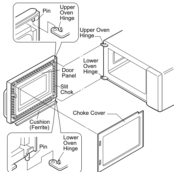
Figure C-7. Door Replacement
